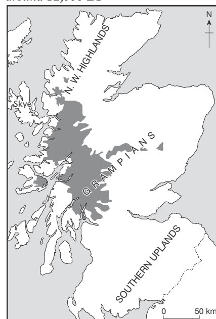
Figure 2: Glaciers and ice-caps (shaded) in Scotland during the Younger Dryas, around 12,000 BP
